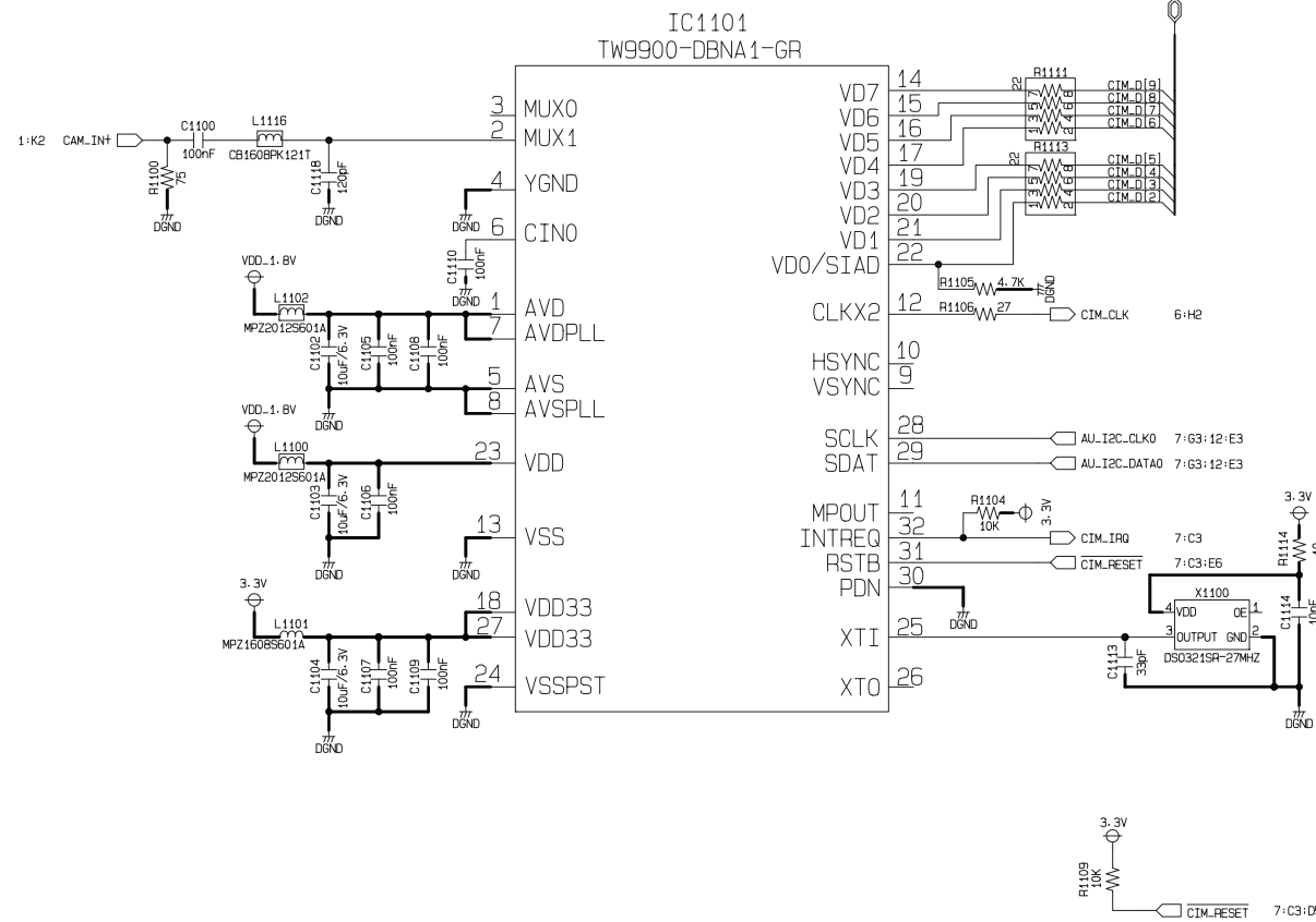
VIDEO DECODER
